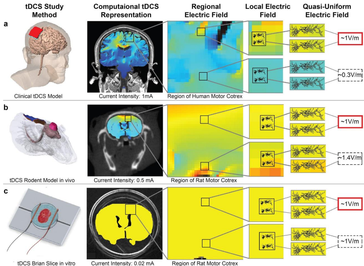
Fig 5.3. The quasi-uniform assumption in modeling and animal studies. A high-resolution finite element method (FEM) computational model of predicted current distribution during tDCS in a slice of the whole brain, a cortical column, and a neuron in (a) Human. (b) Rat In vivo. (c) Rat brain slice in vitro.
